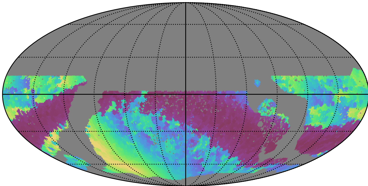
baseline_v3.3_10yrs WFD r band: Min solarElong
