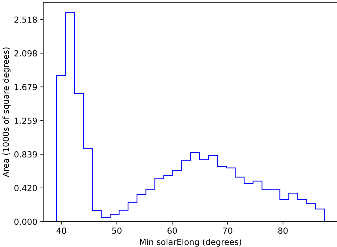
baseline_v3.3_10yrs WFD r band: Min solarElong
