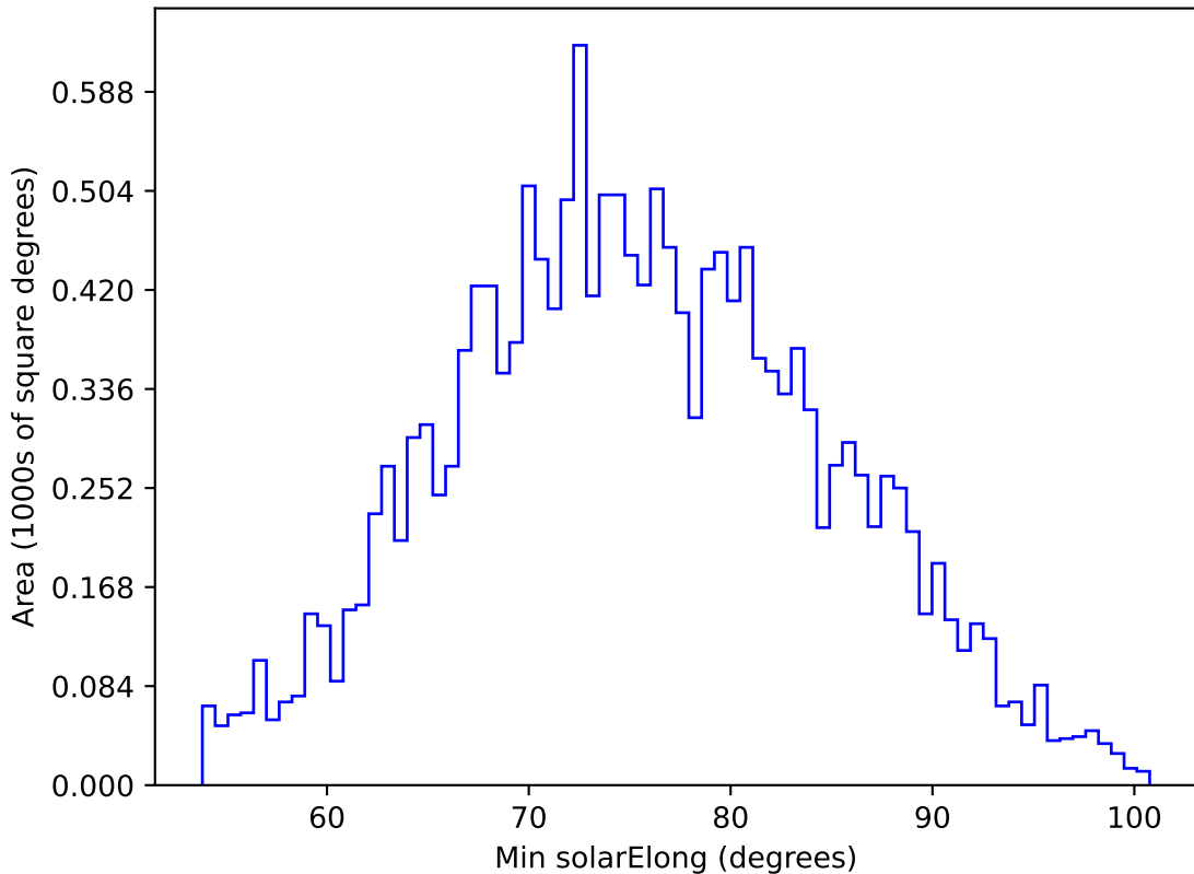
baseline_v3.3_10yrs WFD g band: Min solarElong
