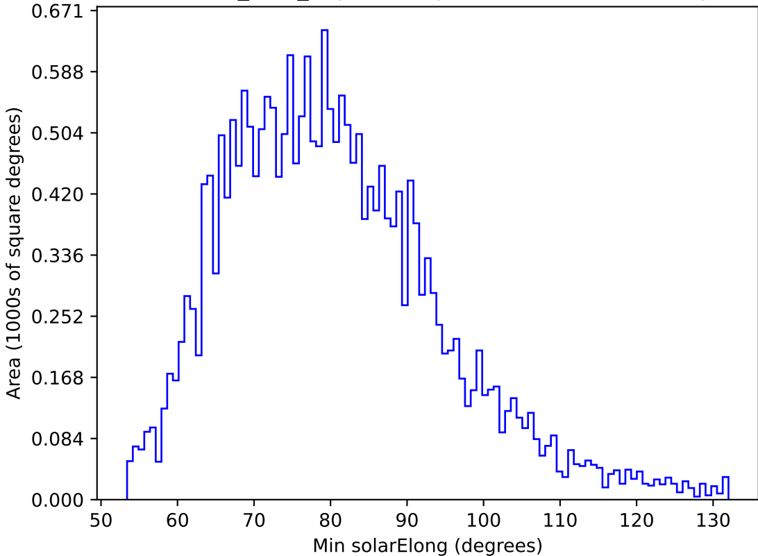
baseline_v3.3_10yrs All sky u band: Min solarElong
