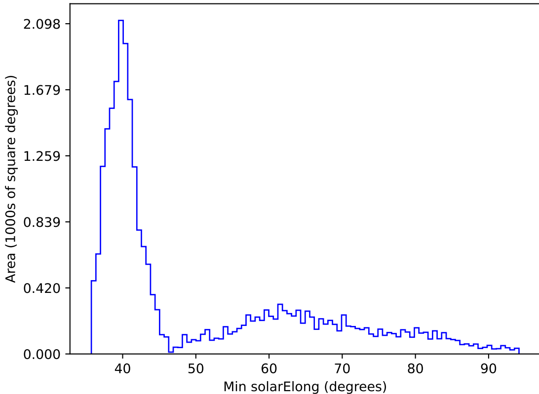
baseline_v3.3_10yrs All sky all bands: Min solarElong
