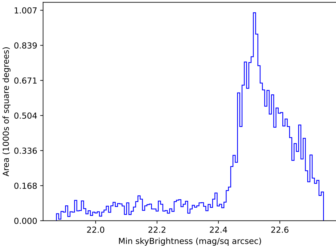
baseline_v3.3_10yrs Yr 1 u band: Min skyBrightness
