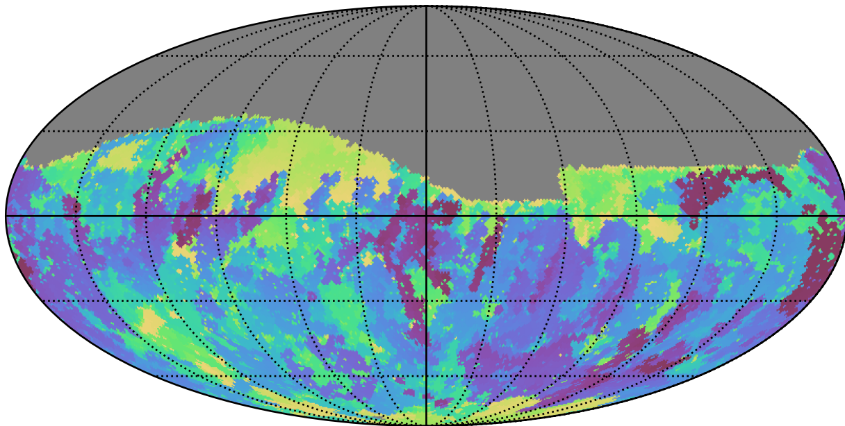
baseline_v3.3_10yrs Yr 1 r band: Min skyBrightness
