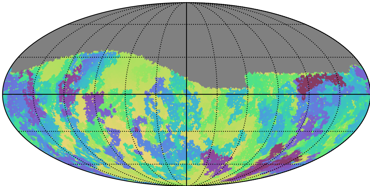
baseline_v3.3_10yrs Yr 1 g band: Min skyBrightness
