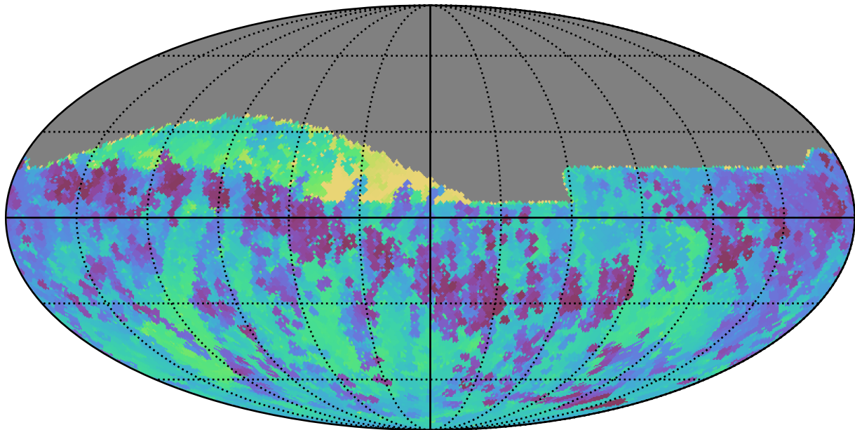
baseline_v3.3_10yrs Yr 1 all bands: Min skyBrightness
