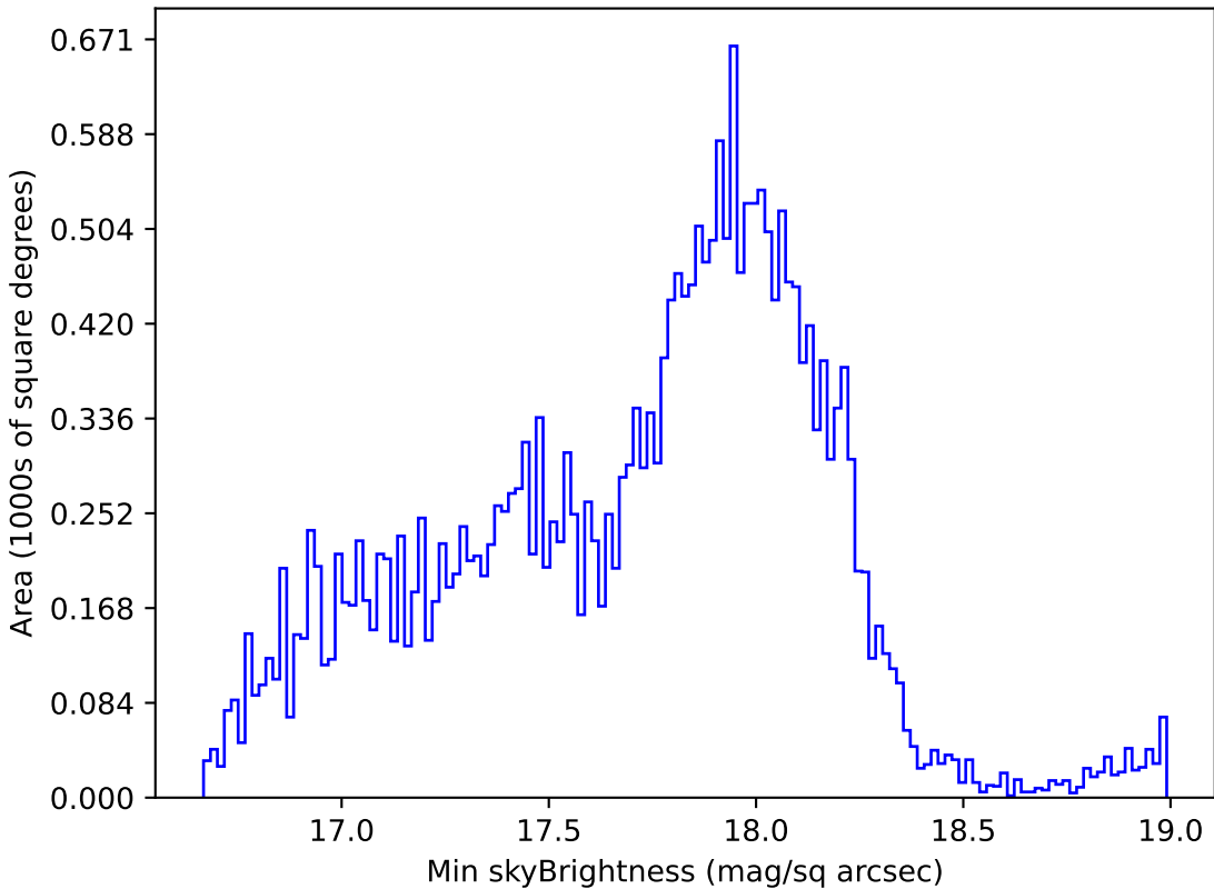
baseline_v3.3_10yrs Yr 1 all bands: Min skyBrightness
