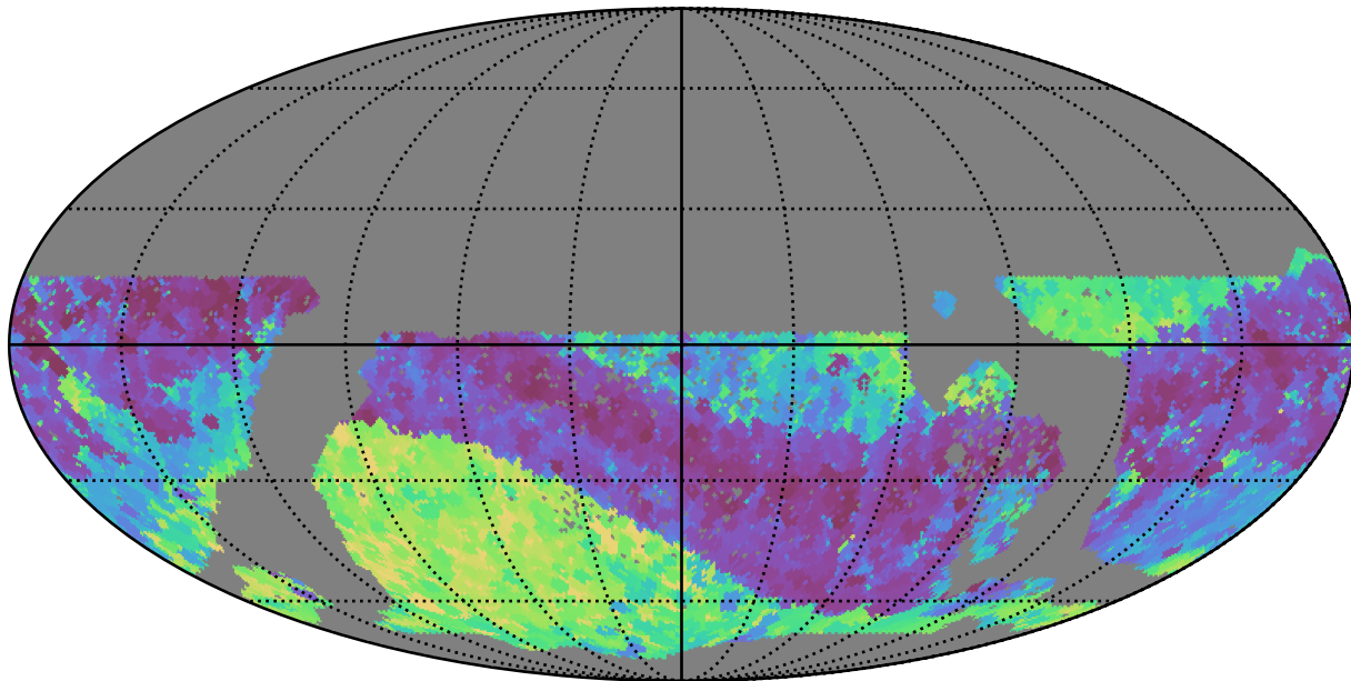
baseline_v3.3_10yrs WFD z band: Min skyBrightness
