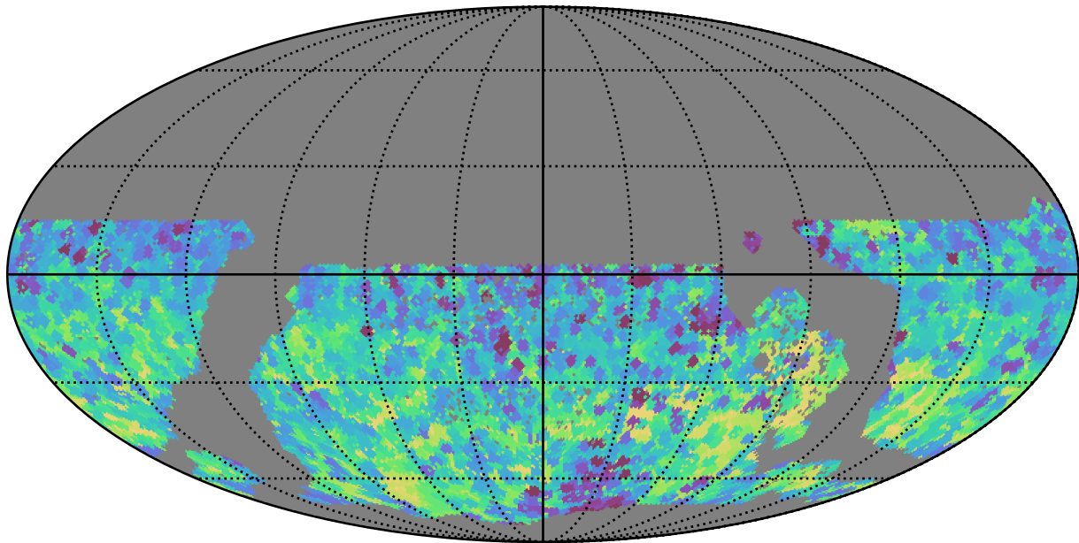
baseline_v3.3_10yrs WFD y band: Min skyBrightness
