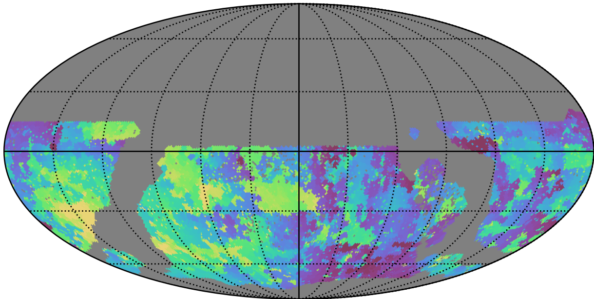
baseline_v3.3_10yrs WFD u band: Min skyBrightness
