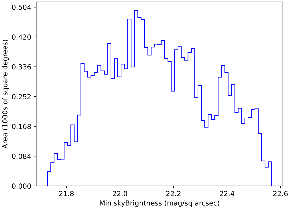
baseline_v3.3_10yrs WFD u band: Min skyBrightness
