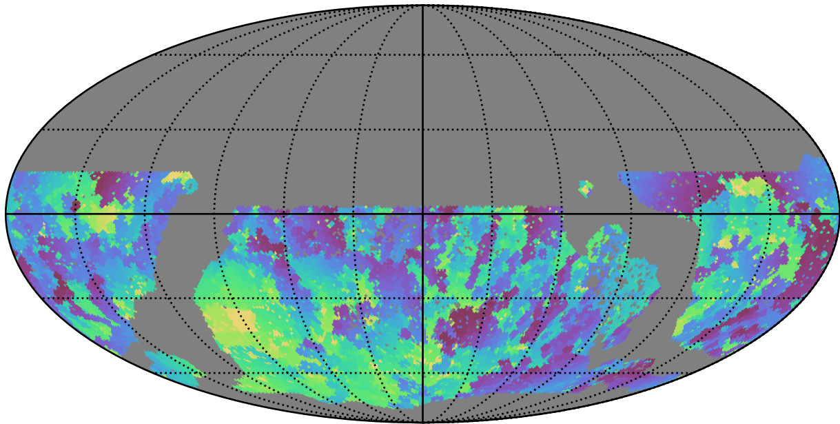
baseline_v3.3_10yrs WFD r band: Min skyBrightness
