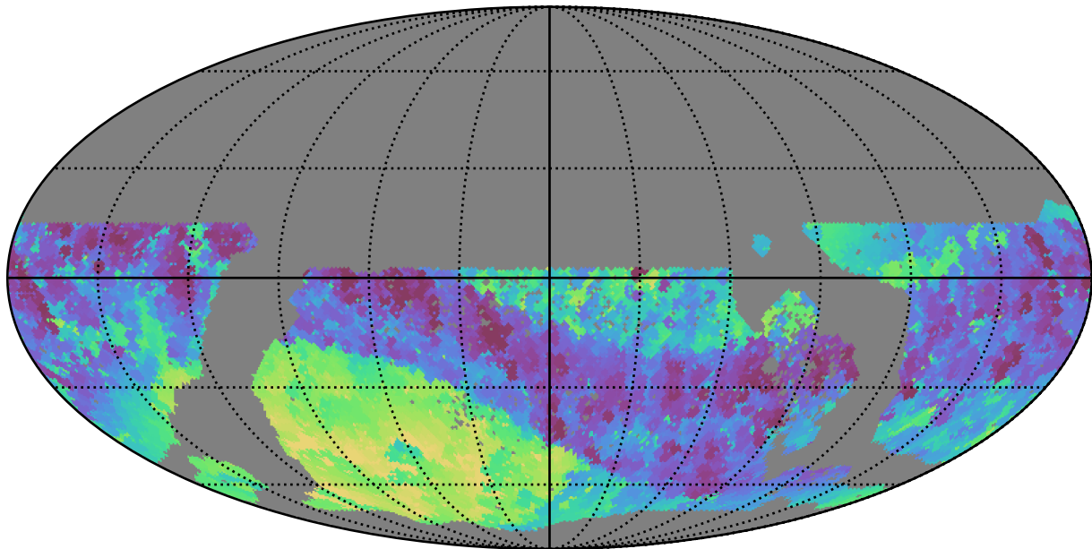
baseline_v3.3_10yrs WFD i band: Min skyBrightness
