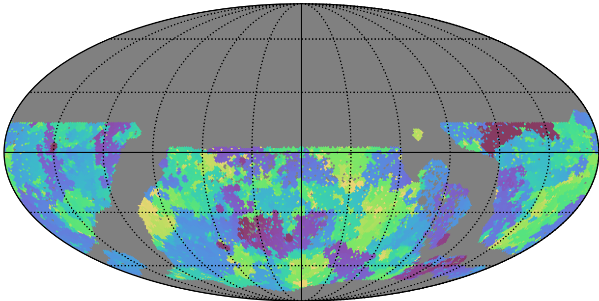
baseline_v3.3_10yrs WFD g band: Min skyBrightness
