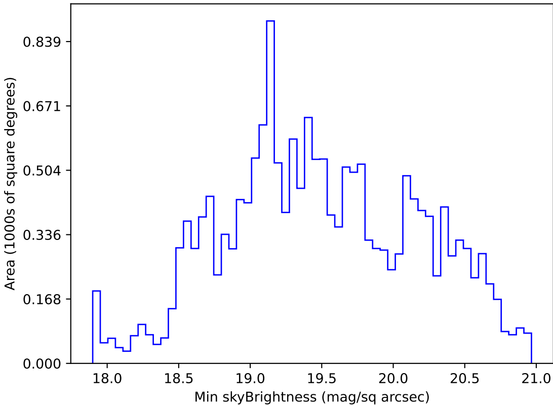
baseline_v3.3_10yrs WFD g band: Min skyBrightness
