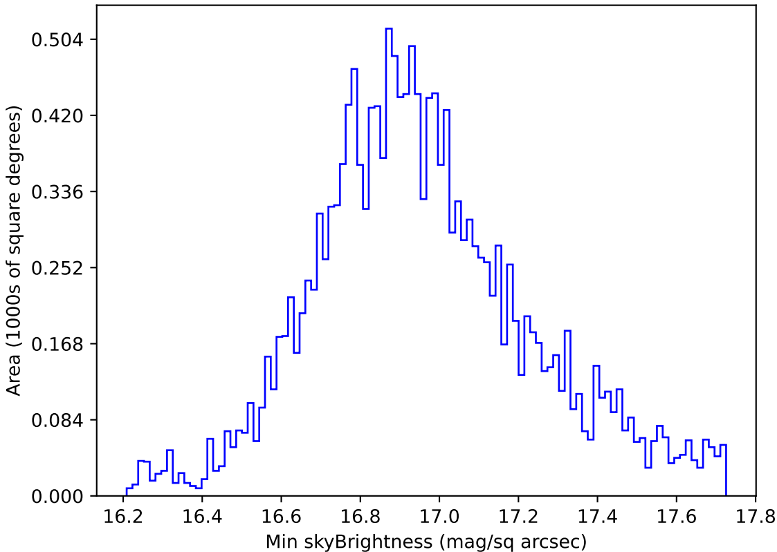
baseline_v3.3_10yrs WFD all bands: Min skyBrightness
