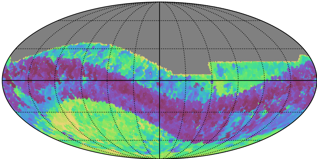
baseline_v3.3_10yrs All sky z band: Min skyBrightness
