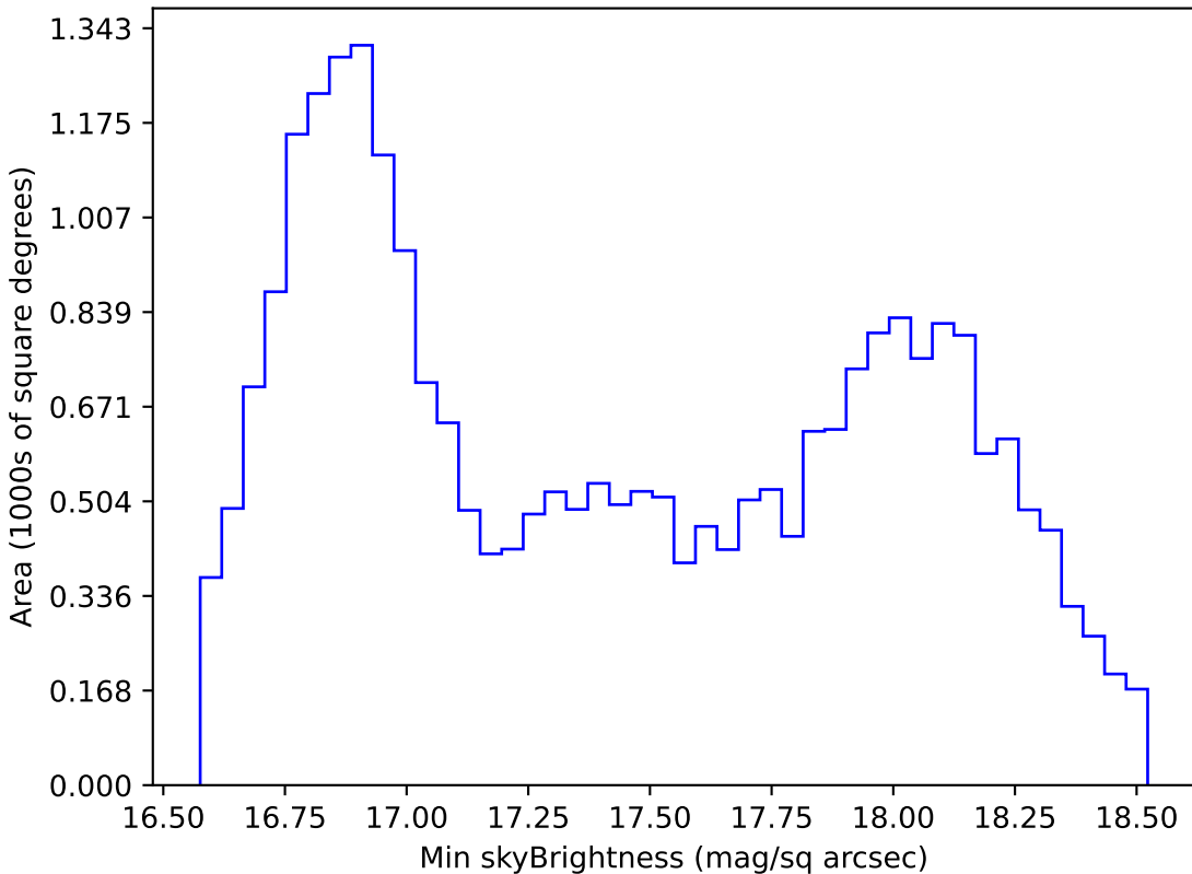
baseline_v3.3_10yrs All sky z band: Min skyBrightness
