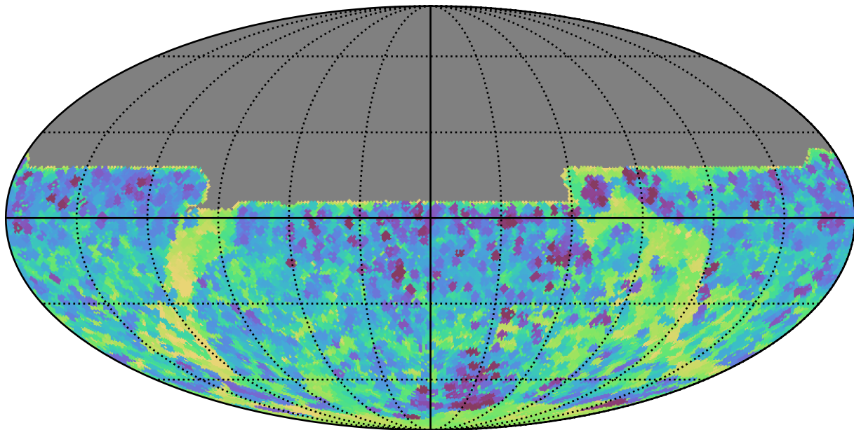
baseline_v3.3_10yrs All sky y band: Min skyBrightness
