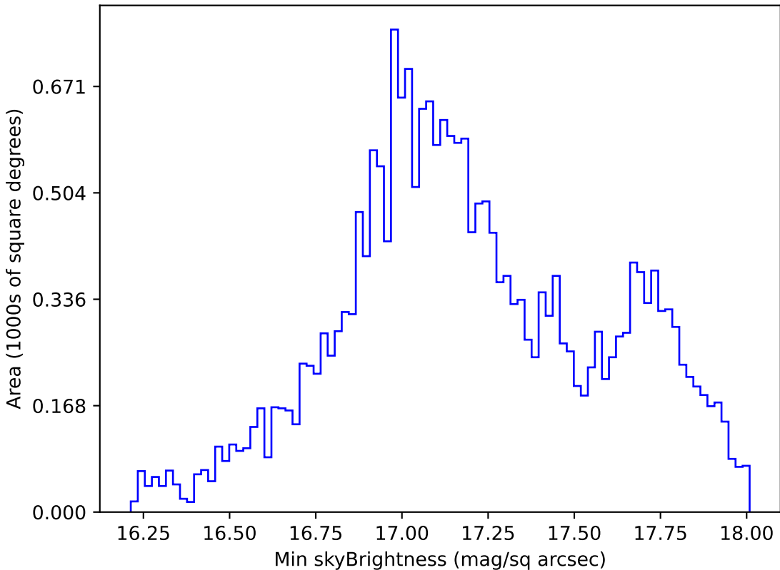
baseline_v3.3_10yrs All sky y band: Min skyBrightness
