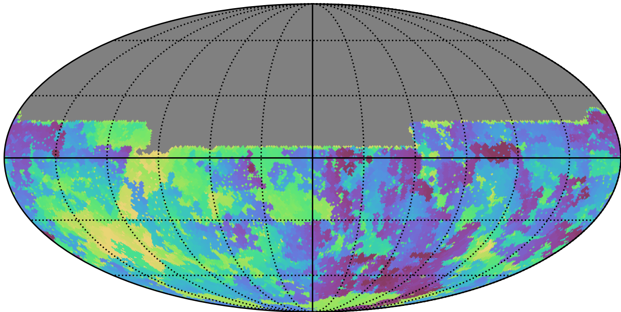
baseline_v3.3_10yrs All sky u band: Min skyBrightness
