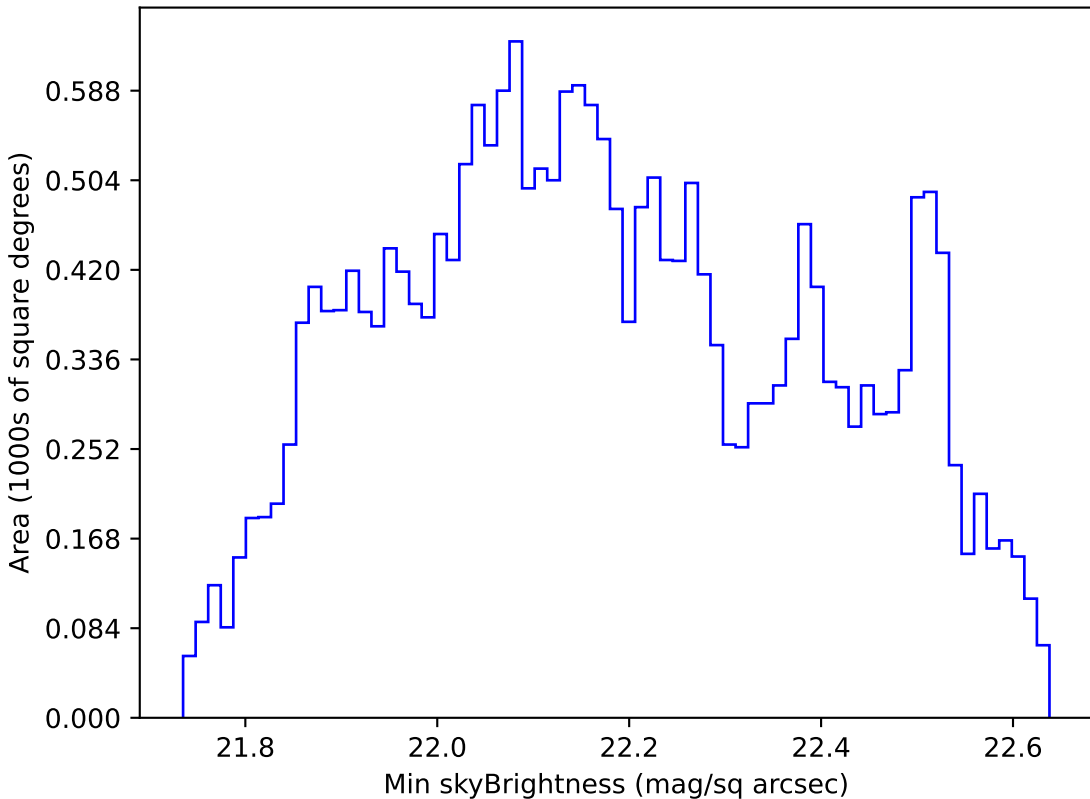
baseline_v3.3_10yrs All sky u band: Min skyBrightness
