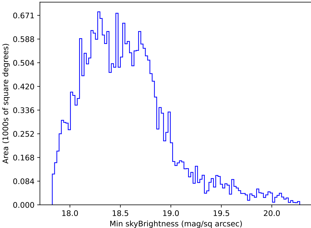
baseline_v3.3_10yrs All sky r band: Min skyBrightness
