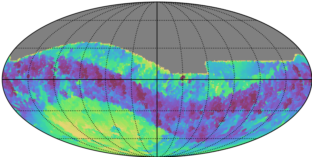
baseline_v3.3_10yrs All sky i band: Min skyBrightness
