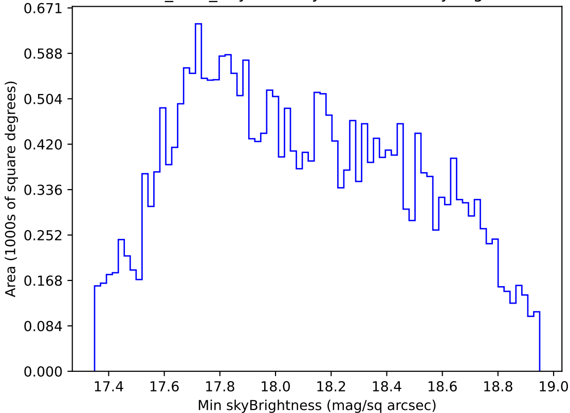
baseline_v3.3_10yrs All sky i band: Min skyBrightness
