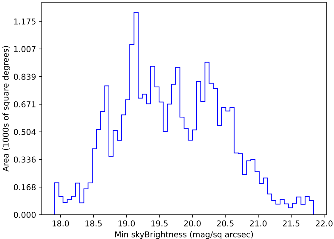
baseline_v3.3_10yrs All sky g band: Min skyBrightness
