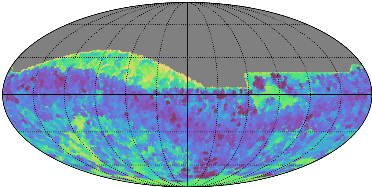
baseline_v3.3_10yrs All sky all bands: Min skyBrightness
