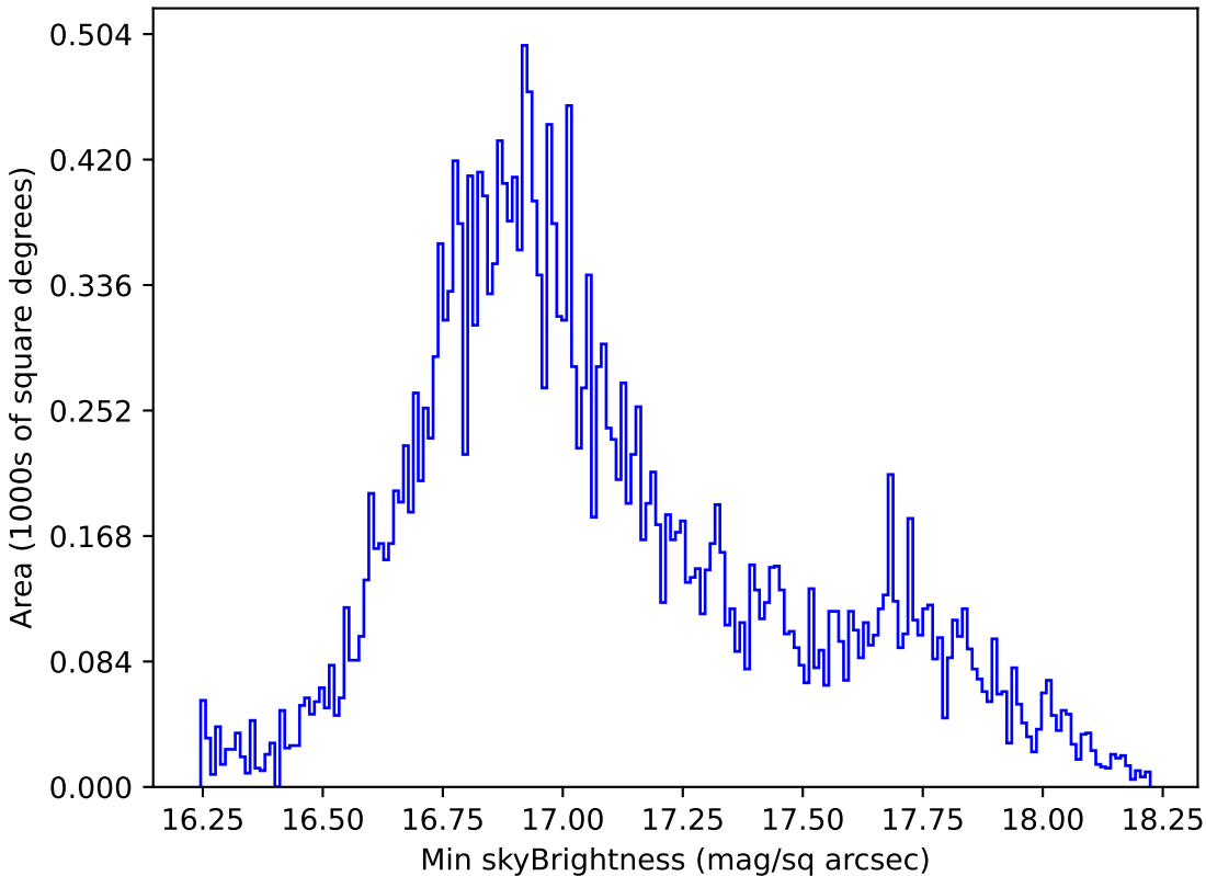
baseline_v3.3_10yrs All sky all bands: Min skyBrightness
