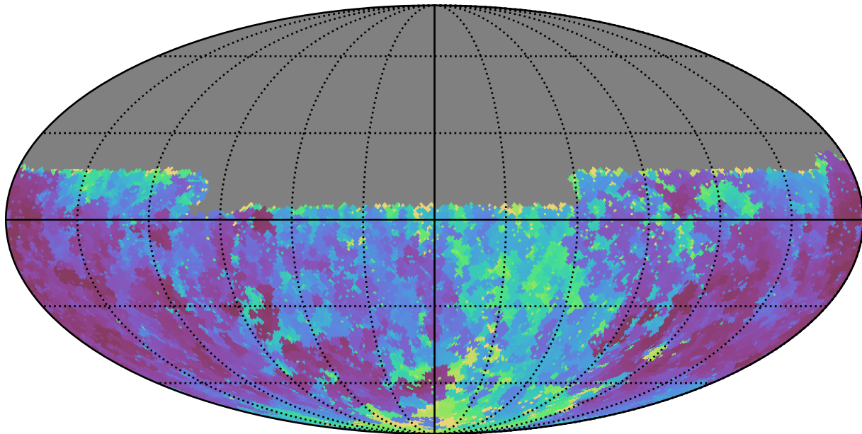
baseline_v3.3_10yrs Yr 1 u band: Min seeingEff
