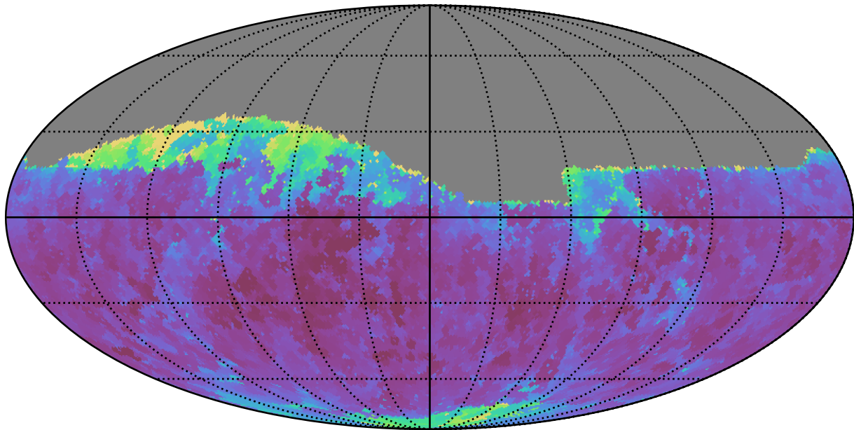
baseline_v3.3_10yrs Yr 1 i band: Min seeingEff
