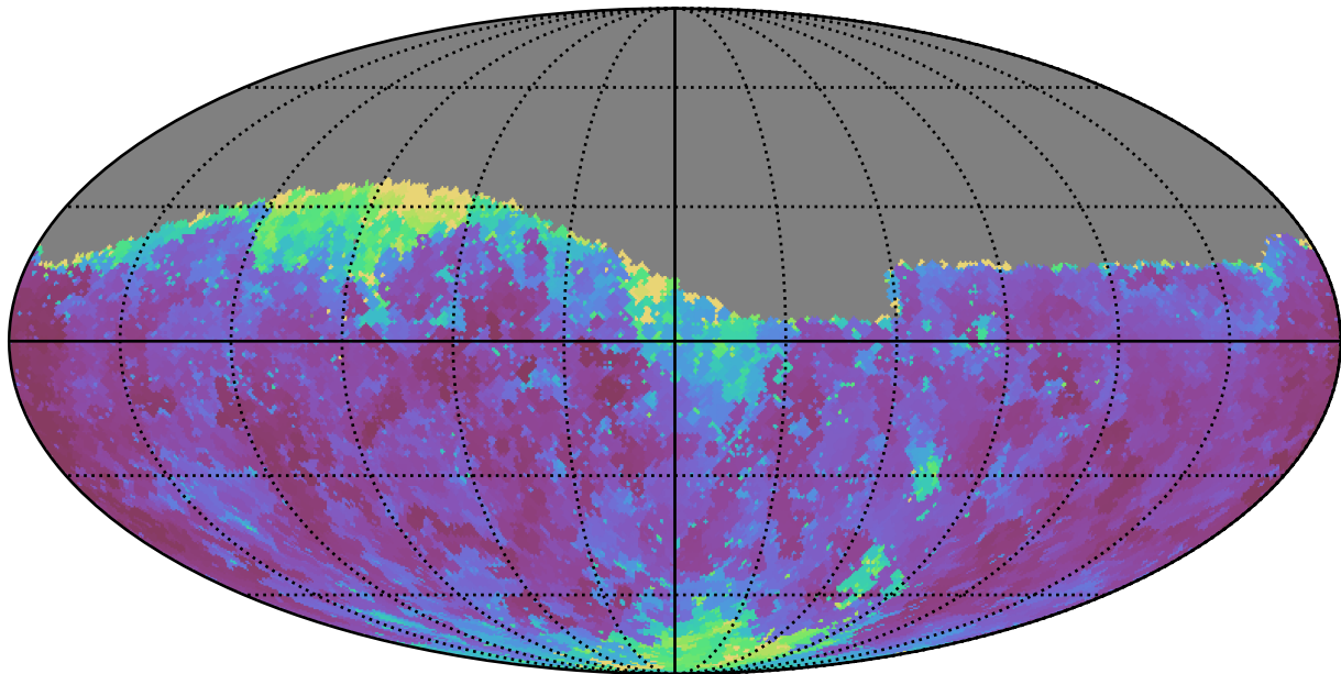
baseline_v3.3_10yrs Yr 1 g band: Min seeingEff
