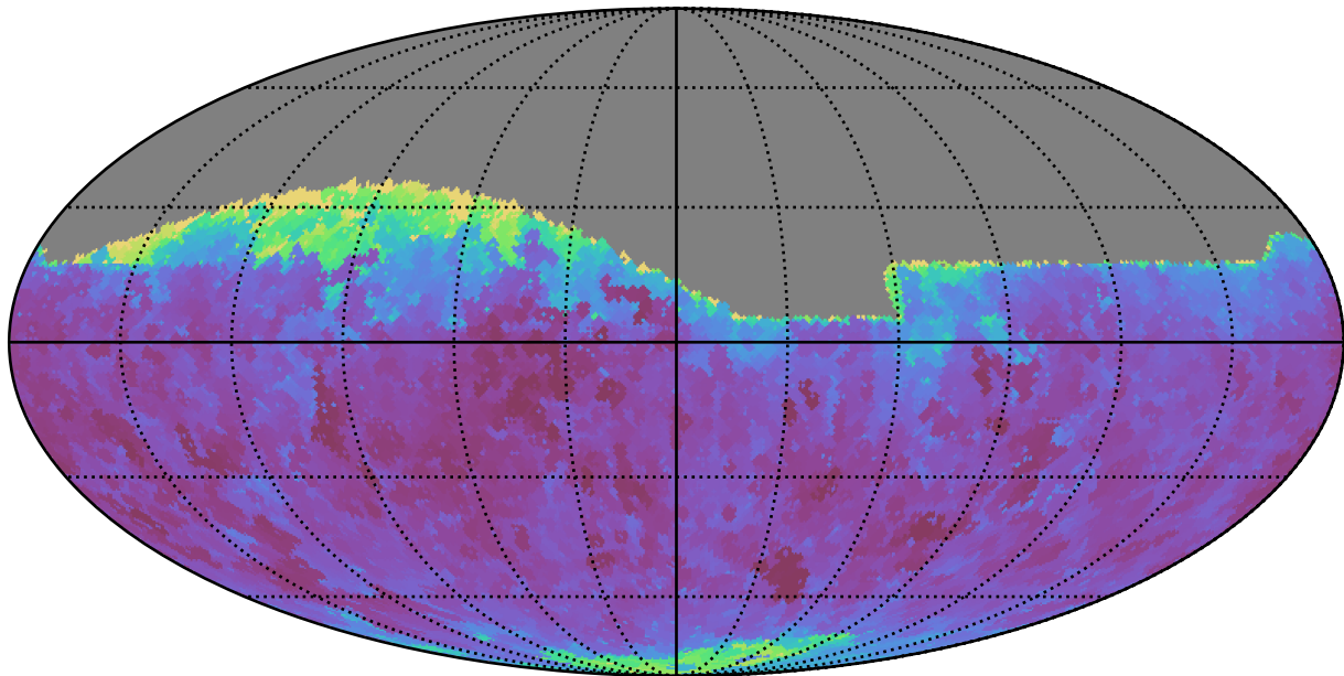
baseline_v3.3_10yrs Yr 1 all bands: Min seeingEff
