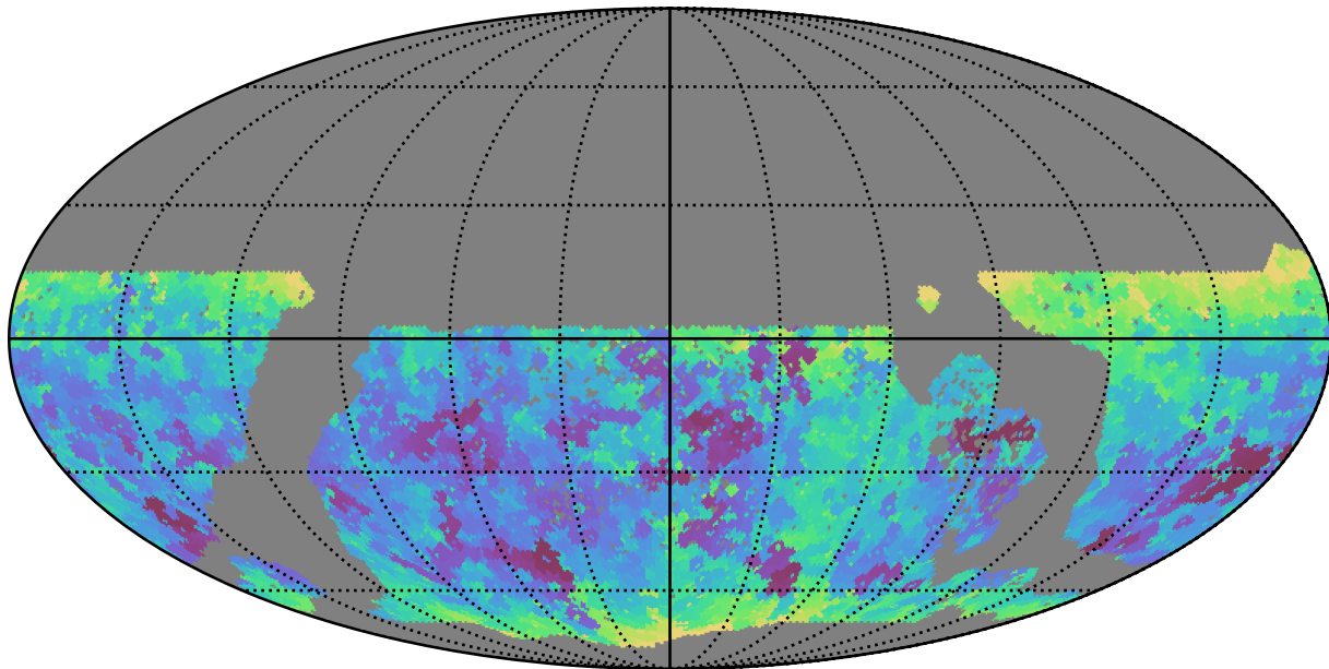
baseline_v3.3_10yrs WFD z band: Min seeingEff
