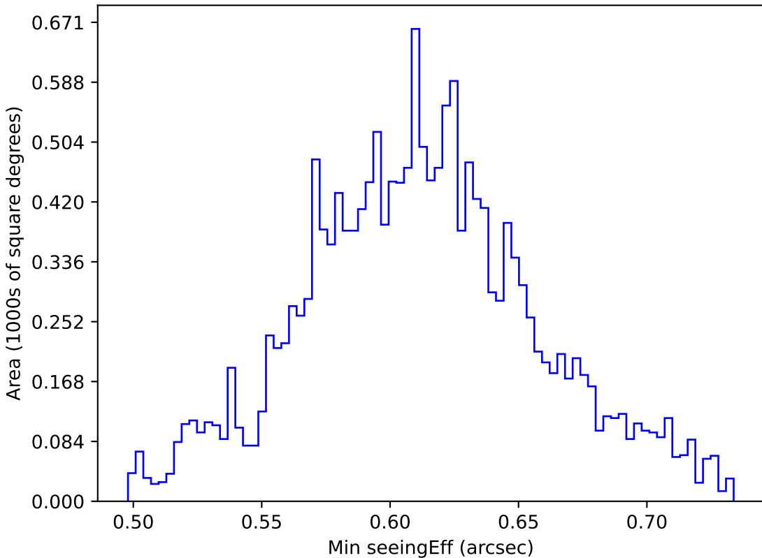
baseline_v3.3_10yrs WFD z band: Min seeingEff
