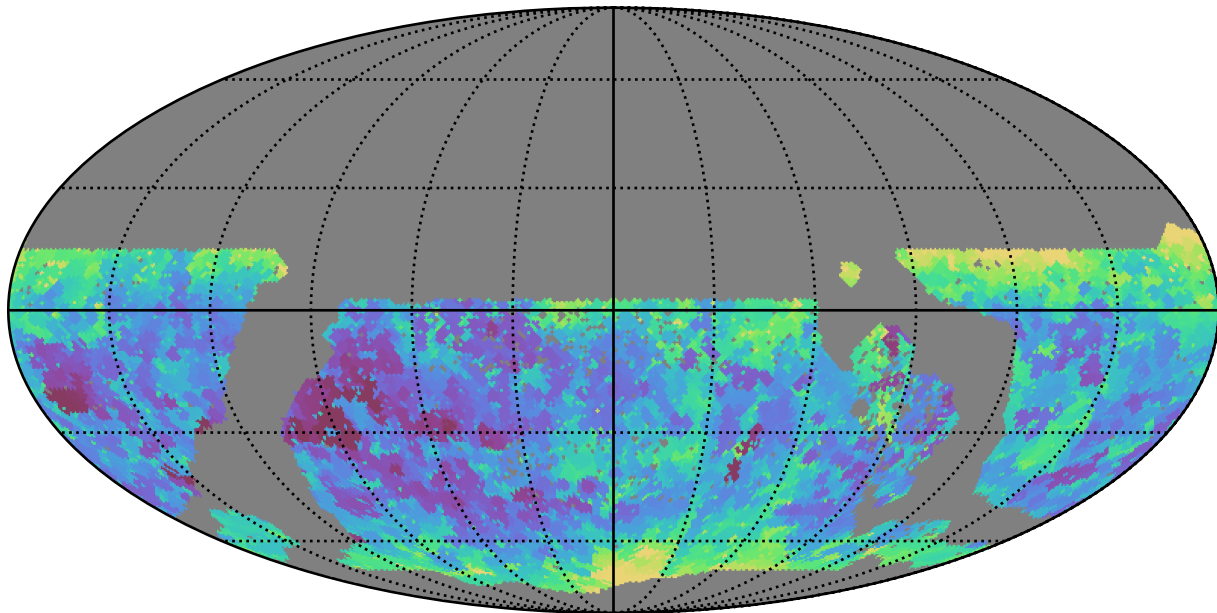
baseline_v3.3_10yrs WFD y band: Min seeingEff
