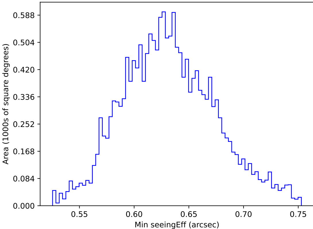
baseline_v3.3_10yrs WFD y band: Min seeingEff
