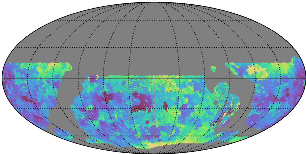
baseline_v3.3_10yrs WFD u band: Min seeingEff
