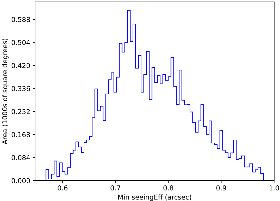
baseline_v3.3_10yrs WFD u band: Min seeingEff
