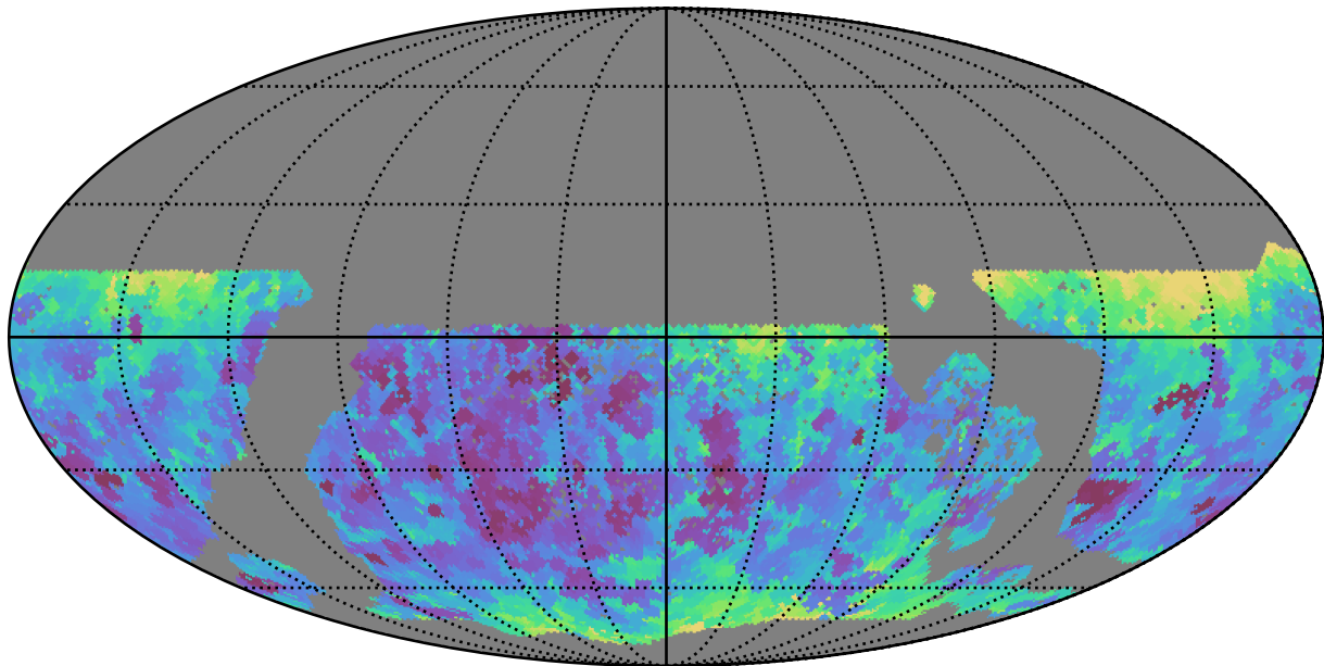
baseline_v3.3_10yrs WFD i band: Min seeingEff
