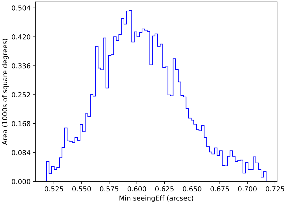
baseline_v3.3_10yrs WFD i band: Min seeingEff
