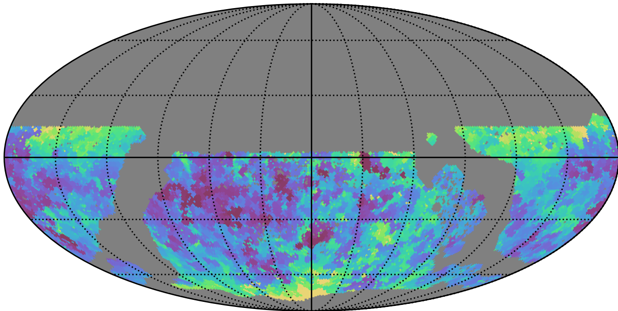
baseline_v3.3_10yrs WFD g band: Min seeingEff
