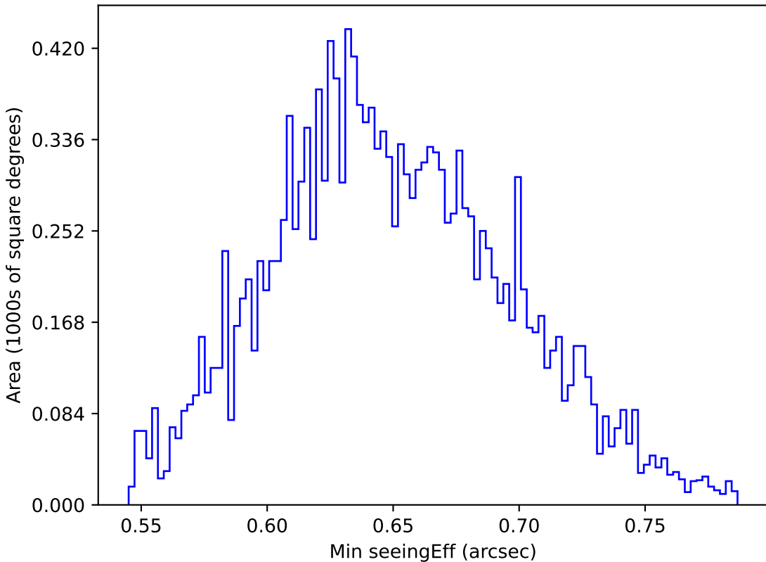
baseline_v3.3_10yrs WFD g band: Min seeingEff
