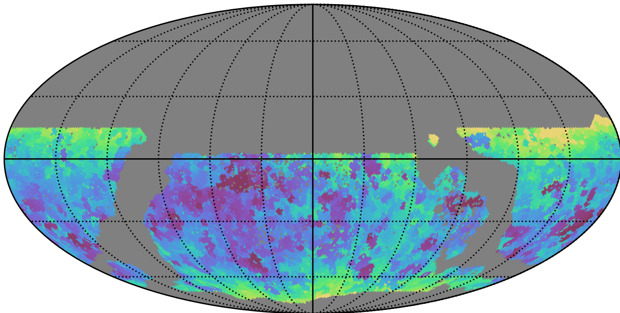
baseline_v3.3_10yrs WFD all bands: Min seeingEff
