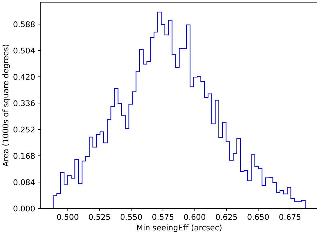
baseline_v3.3_10yrs WFD all bands: Min seeingEff
