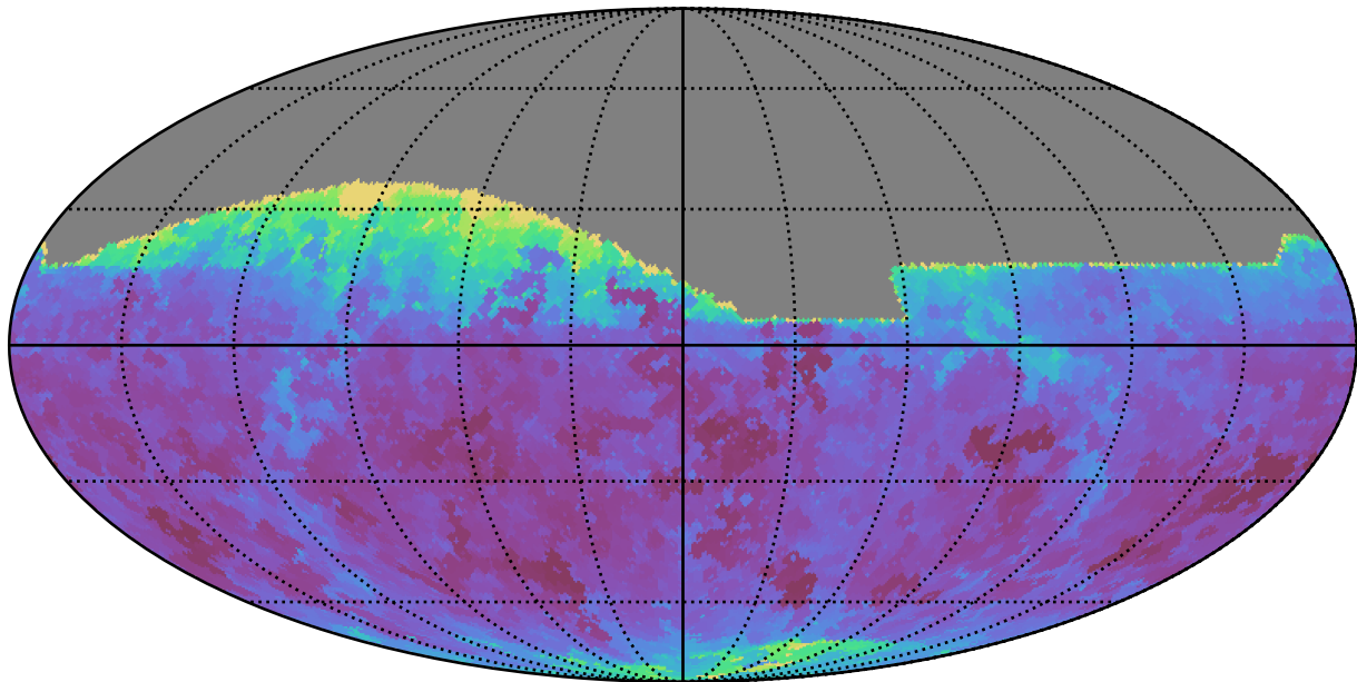
baseline_v3.3_10yrs All sky z band: Min seeingEff
