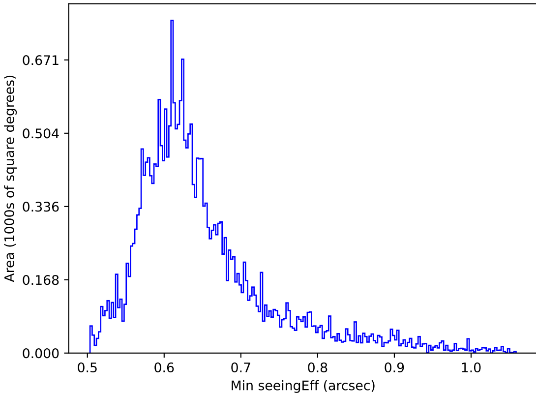
baseline_v3.3_10yrs All sky z band: Min seeingEff
