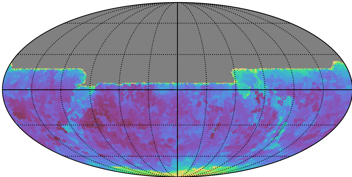
baseline_v3.3_10yrs All sky y band: Min seeingEff
